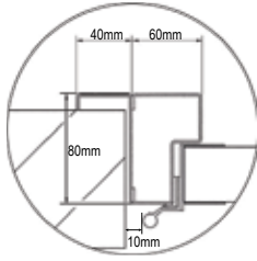
Frame dimensions
