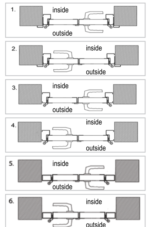
Side Hinged Garage Door fitting and handing options (also available opening inwards)
